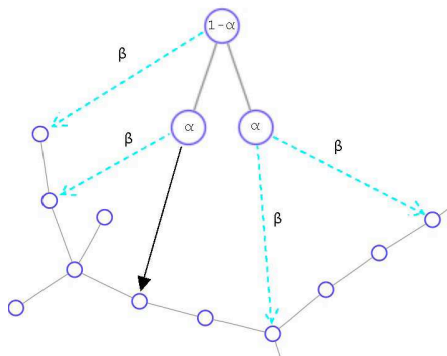
Fig. 3: (Color online) Illustration of the \mathcal{V}_\beta model. Once the graphlet attaches to the network, based on \alpha , we introduce up to l (here l = 4 ) additional edges from the graphlet into random nodes of the network, each with probability \beta .
